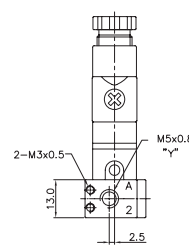
YSV221-DP-SC1-CN1-*** Normally Open
