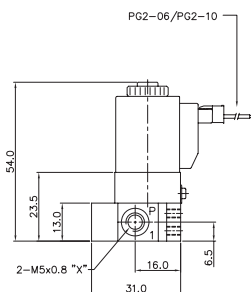
YSV211-DP-SL1-*** Normally Closed
