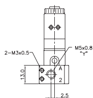
YSV221-DP-SG1-*** Normally Open
