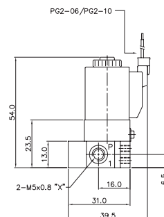
YSV211-DP-SM1-*** Normally Closed
