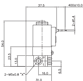
YSV211-DP-SD1-*** Normally Closed
